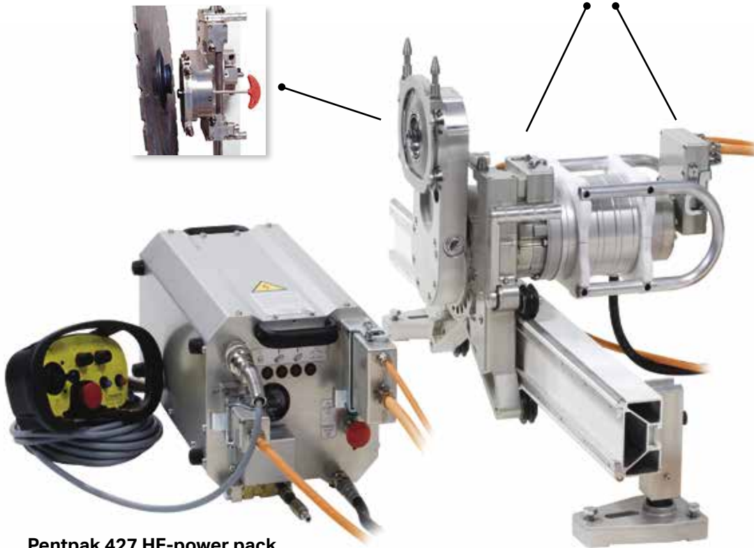
Pentpak 427 HF-power pack with Pentrunder autofeed system
